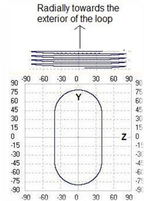
Figure 3 (radial drift on a figure of "0")
